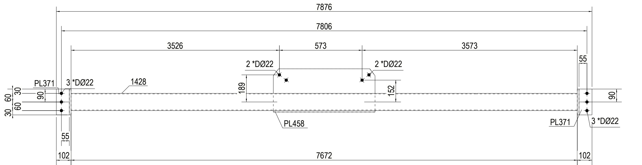
FRONT VIEW
